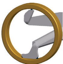
Tasterform / probe contacts 1 Kugel / Ball Ø 0,6mm
